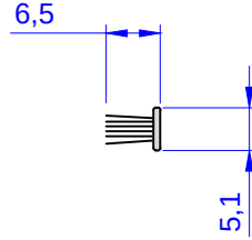
SÜRME KIL FİTİL (51X65) SLIDING WEATHER STRIP
